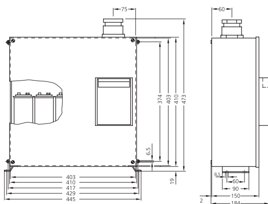
Dimensional drawing LKSLT Case type 1 (7.5 to 40 kvar) All dimensions in mm
