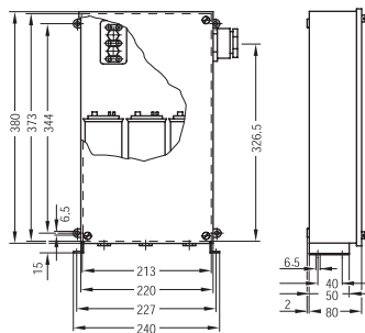
Dimensional drawing LKN Case type 2 (12.5 to 15 kvar)
