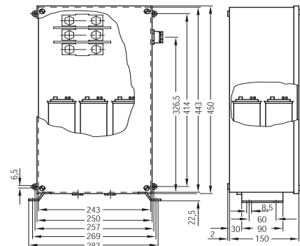
Dimensional drawing LKN Case type 3 (20 to 30 kvar)
